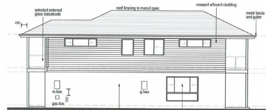
ELEVATION 2 SCALE 1:100
