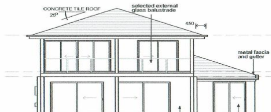
ELEVATION 3 SCALE 1:100
