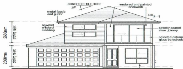
ELEVATION 1 SCALE 1:100
