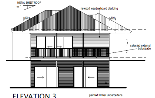
ELEVATION 3 SCALE 1:100
