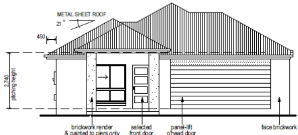
ELEVATION 1 SCALE 1:100
