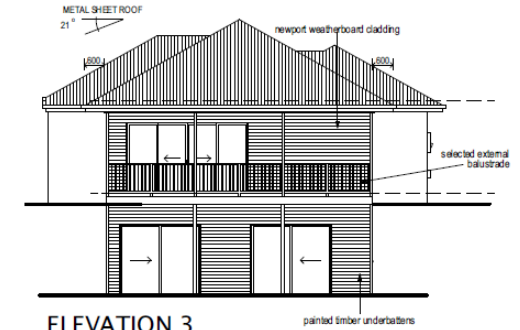
ELEVATION 3 SCALE 1:100
