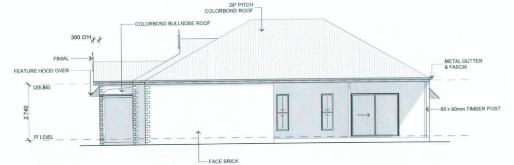
B RIGHT ELEVATION Scale 1:100
