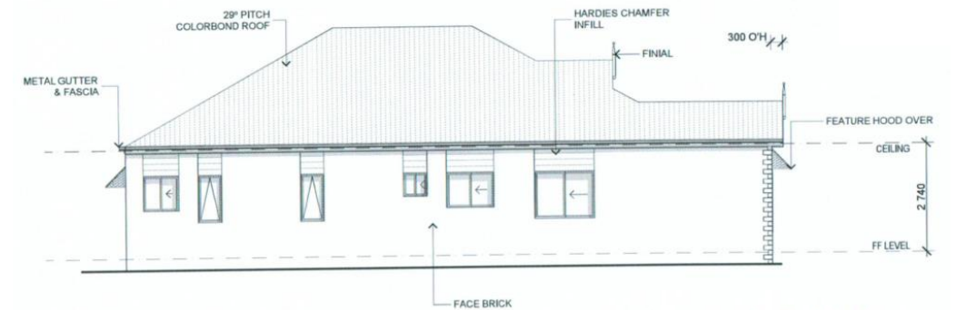
C LEFT ELEVATION Scale 1:100
