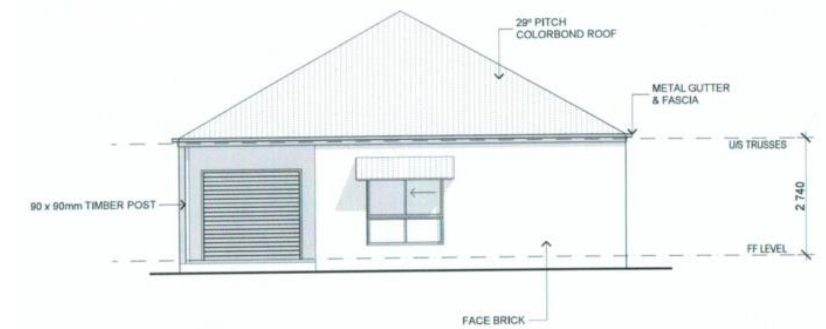
D REAR ELEVATION Scale 1:100
